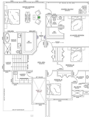
UPPER FLOOR SCALE: 1/4" = 1'-0"
