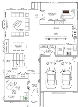
MAIN FLOOR P1 SCALE: 1/4" = 1'-0"
