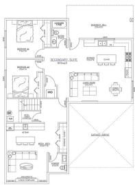
BASEMENT FLOOR SCALE: 1/4" = 1'-0"
