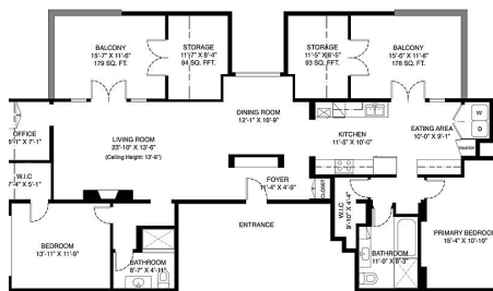
MAIN FLOOR PLAN Ceiling Height: 8'-3"
